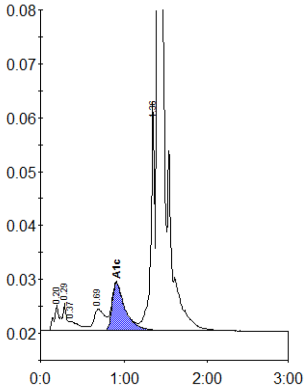
Peak table - ID: 10661762
